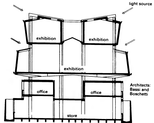
7 Section and light sources Museo Civico, Turin
